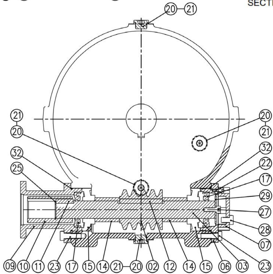
SECTION B-B
